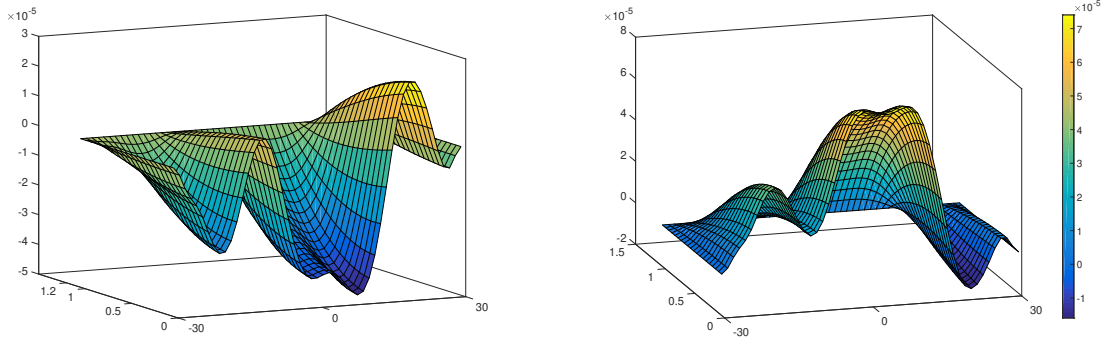
FIGURE 2. Disturbance signal \psi (left) and control function v (right) on the spatial domain (-30, 30) . T = 1s , N = 50 , \Delta t = 2 \times 10^{-2} and \ell = 40 , \gamma = 40 .
