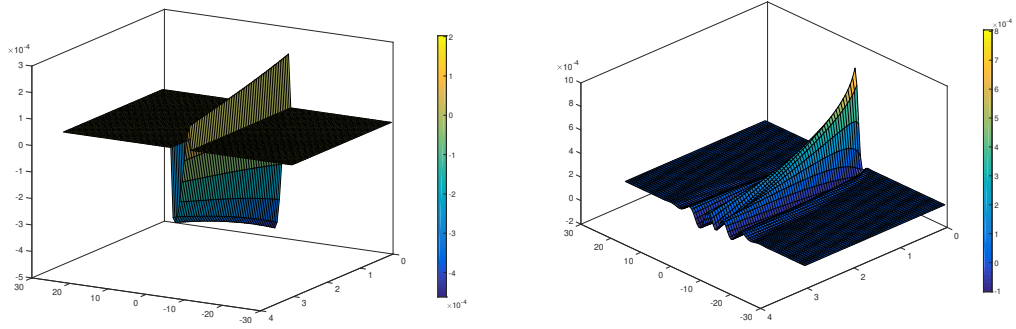
FIGURE 10. Lider (left) and state (right). T = 3s, N = 100, \Delta t = 2 \times 10^{-2}, \ell = \gamma = 40 . Domains \omega = (-3, 1) and \mathcal{O} = (-1, 3) , initial datum u_0(x) = 10^{-3} \exp(-x^2) .
