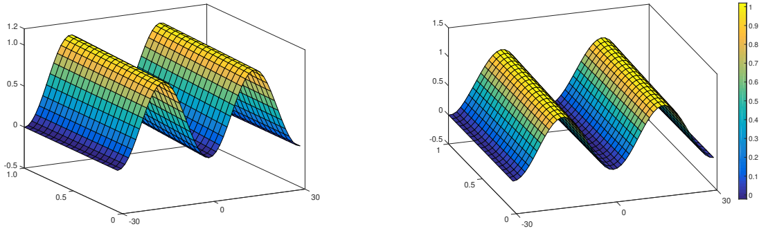
FIGURE 3. Function u_d(x, t) = \sin^2(\frac{\pi x}{30}) + 10^{-1}t(\cos(\frac{\pi x}{30}) + 1) (left) and state function u(x, t) (right). T = 1s , N = 50 , \Delta t = 2 \times 10^{-2} and \ell = 40 , \gamma = 40 .
